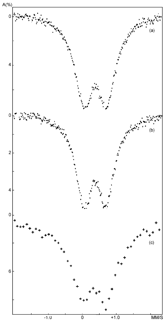
FIGURE 3 Room temperature Mössbauer spectra of (a) alginate magnetic composite, (b) starch magnetic composite, and (c) chitosan magnetic composite.
